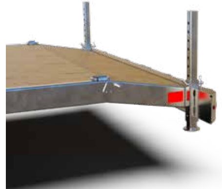
STABILIZER LEGS
