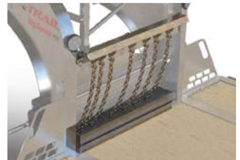
STANDARD CHAIN TRAY
